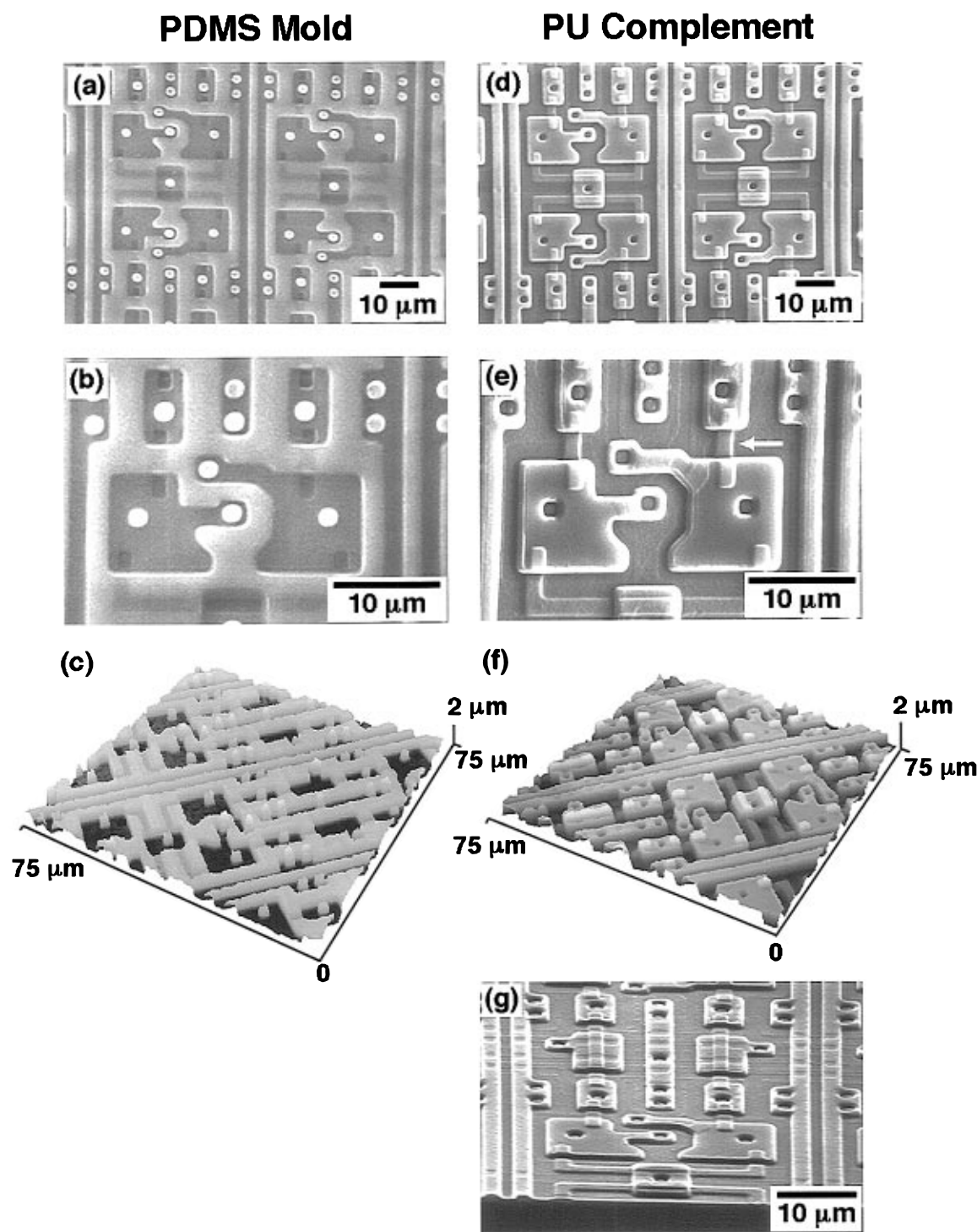
Figure 2. Comparison of a PDMS mold with a topologically complex surface and the complementary PU structure made against it using MIMIC. (a, b) SEM images of the PDMS mold at two different magnifications. (c) AFM image of the PDMS mold. (d, e) SEM images of the corresponding PU microstructures formed on a Si/SiO 2 surface. The patterned PU layer has features with different thicknesses; the thinnest parts of the layer (indicated by the arrow in (e)) are less than 100-nm thick. (f) AFM image of the PU complement. (g) Fracture view by scanning electron microscopy (at 60°) of the PU layer.
