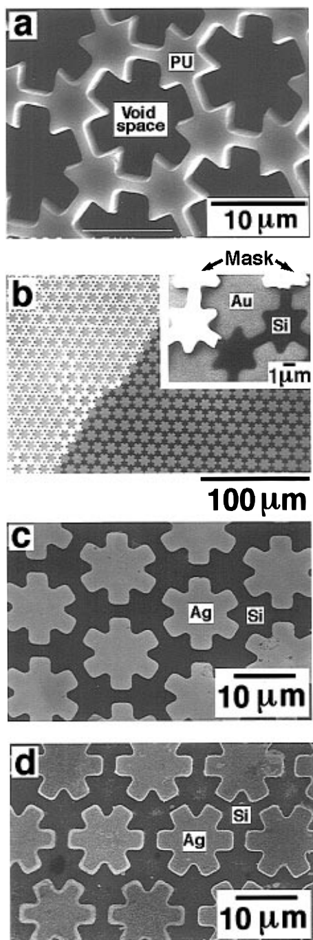
Figure 10. (a) SEM image of a free-standing PU microstructure that was used subsequently as the disposable mask for patterning different substrates using evaporation of metals or formation of SAMs. (b) SEM of a planar Si/SiO 2 surface that had been patterned with gold by evaporation through the mask. In this picture, half of the mask still remained on the surface. The inset is a blowup to show the edge resolution of this pattern. (c, d) SEMs of patterned features of silver (bright regions) that were generated on a Si/SiO 2 surface by selective etching using patterned SAMs of hexadecanethiolate as resists that were formed using free-standing PU films as the masks (see text for detail).
