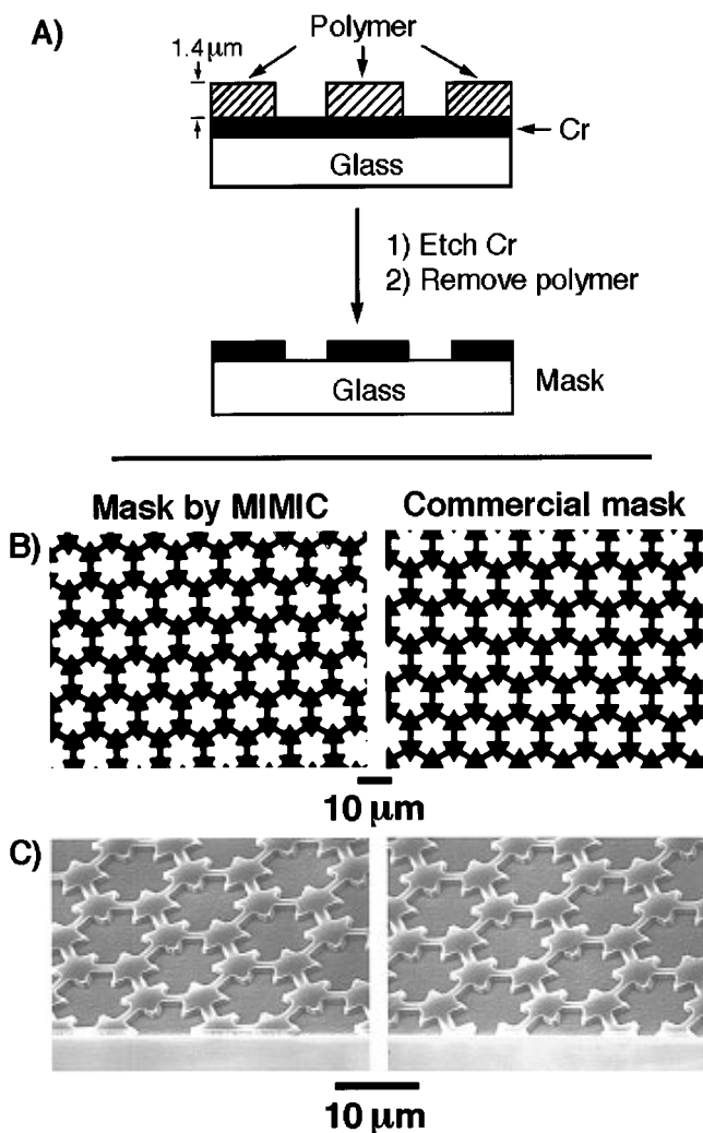
Figure 8. (A) Schematic procedure that was used to fabricate chrome-masks using MIMIC. (B) Optical micrographs of the chrome-masks that were produced using MIMIC and the conventional method, respectively. (C) SEM images of a test pattern that was generated in positive-tone photoresist films (Microposit 1813, Shipley) by photolithography using the newly fabricated mask (made using MIMIC) and the commercial chrome mask, respectively.
