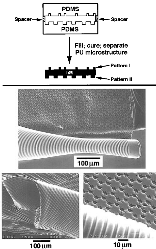
Figure 4. SEM images of a free-standing microstructure of PU that was formed between two PDMS molds that had different relief patterns in their surfaces and were separated by a certain distance using a spacer (Scotch tape) when carrying out MIMIC. After filling the channels and curing the PU prepolymer into a cross-linked polymer, the two PDMS mold were separated; the PU microstructures remained in one of the molds and could be released using tweezers.
