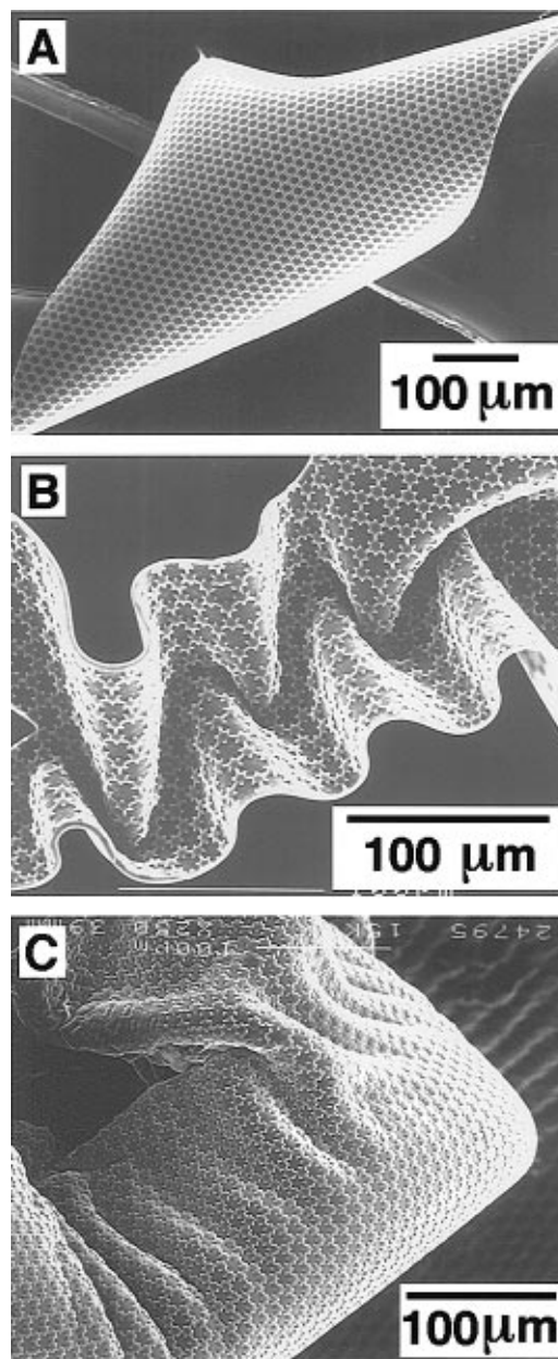
Figure 5. SEM images of patterned PU microstructures that were formed using MIMIC on films of Saran Wrap. These patterned films folded into different shapes; the PU microstructures adhere well and roughly retained their forms. The strips (A, B) were produced accidentally on certain regions of the samples when folding the films mechanically.
