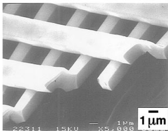
Figure 3. SEM images (at three different magnifications) of a free-standing polymeric (PU, J-91) microstructure that was formed between two PDMS molds. Each mold has a relief pattern of parallel lines in its own surface. The free-standing microstructure was placed on a piece of Scotch tape (there was a hole in the tape, just under the polymeric microstructure, to demonstrate that the microstructure had the structural stability to stand without support) using tweezers. The sizes of features in regions I, II, and III are different, as a result, the electron interference patterns (Moiré effect) from these three regions are different. The two blowups were taken from region I.
