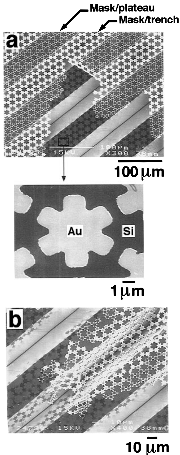
Figure 12. SEM images of contoured surfaces anisotropically etched in Si that were patterned with microfeatures of gold ( \sim 120 nm thick) by evaporation using free-standing polymeric structures as the masks. (a) Mask with a frame was placed on the surface using tweezers; (b) mask without a frame was placed on the surface by floating the mask on water and picking up by the substrate from underneath.
