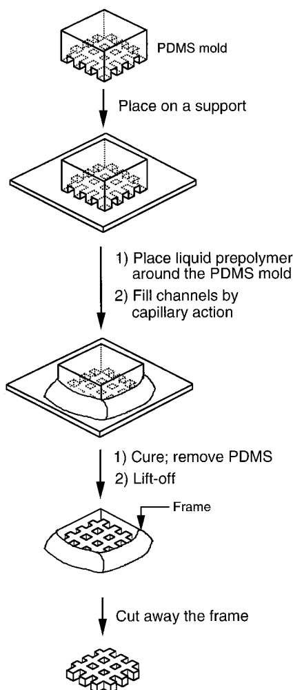
Figure 1. Schematic illustration of MIMIC. After filling the network of channels with a liquid prepolymer, the prepolymer was cured either thermally or photochemically. The PDMS mold was then peeled away carefully. The patterned polymeric microstructure remained on the support and could be released from the surface of the support by dissolving the support.
