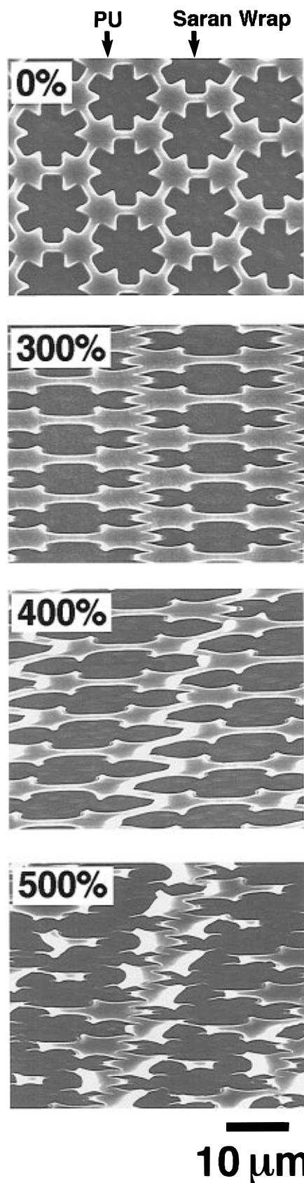
Figure 6. SEM images of a test structure of PU that was formed on films of Saran Wrap using MIMIC and then stretched along the horizontal direction. The stretched forms were fixed using Scotch tapes. As the underlying film of Saran wrap was elongated, the PU structure deformed accordingly. The PU structures broke and became unrecognizable at an elongation of \sim 500\% .
