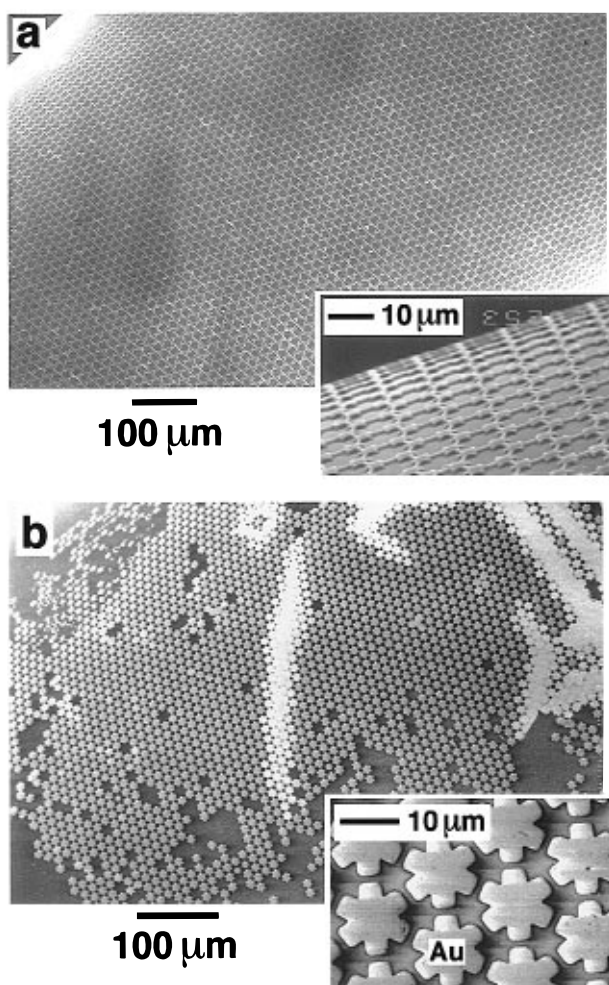
Figure 11. (a) SEM images of a glass capillary (the radius of curvature is ~400 μm) that was covered by the polymeric mask and was exposed to gold by evaporation for ~5 min. The image is of the mask resting on the capillary, with both mask and glass covered with gold. (b) SEM images of the glass capillary of (a) after removing the polymeric mask by dipping the capillary in an aqueous KOH/2-propanol solution at 65 °C for ~2 min. Gold patterns (~100 nm thick) were formed on the glass capillary. The inset is the blowup of the corresponding SEM image.
