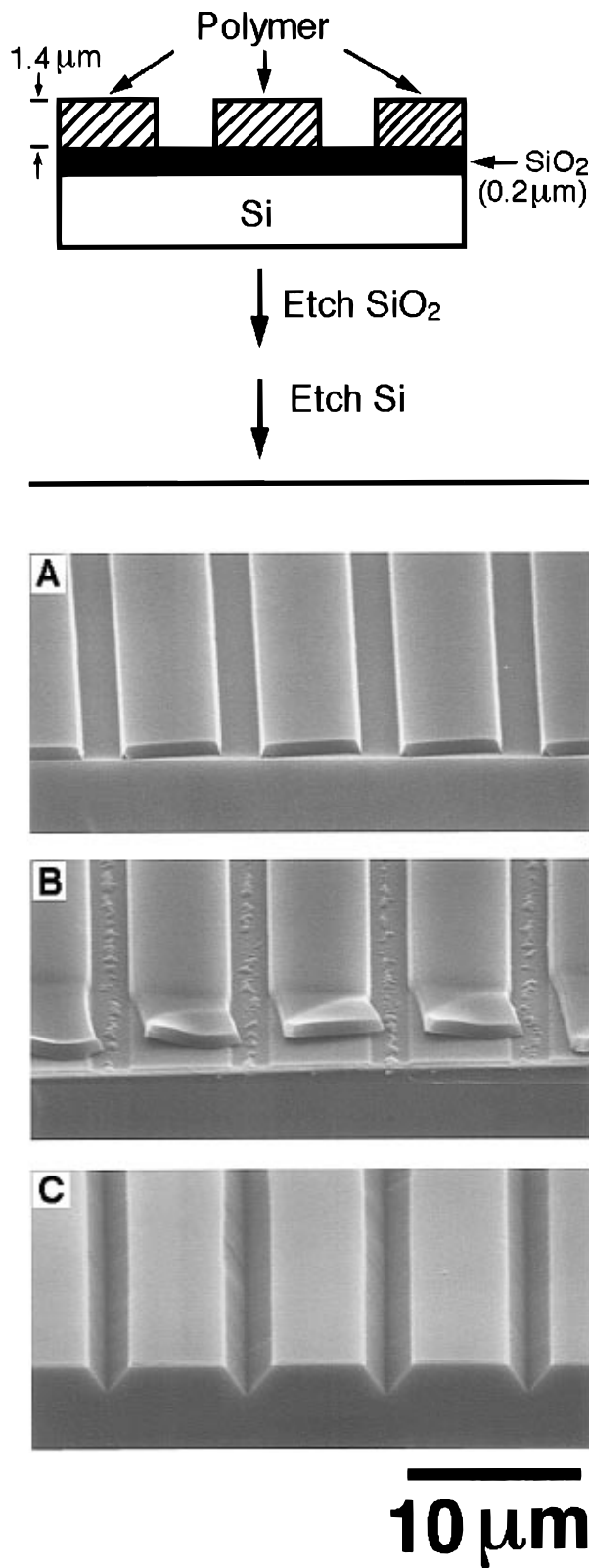
Figure 7. (A) SEM image of a test pattern of PU formed using MIMIC on a silicon wafer covered by thermally-formed \text{SiO}_2 (0.2 \mu\text{m} thick). (B) SEM image of this sample after etching in an aqueous \text{HF}/\text{NH}_4\text{F} solution for \sim 2 min. The ends of the polymer strips deadhered on fracturing the silicon substrate. (C) Same sample as (B) after further etching in an aqueous \text{KOH}/2 -propanol solution for \sim 15 min at 65^\circ\text{C} . The PU structures dissolved or lifted off in the \text{KOH}/2 -propanol solution at this temperature.
