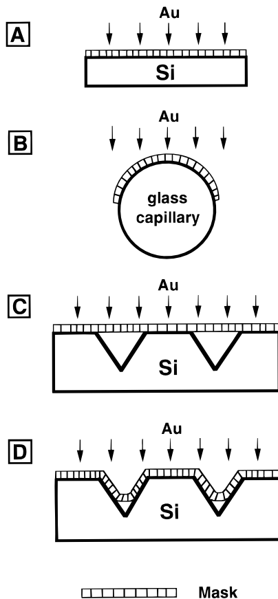
Figure 9. Schematic illustration of evaporation of gold through a patterned polymeric mask onto a planar (A), curved (B), or contoured surface (C, D). The masks used in this procedure were thin ( \sim 1.5 \mu\text{m} ) free-standing microstructures of PU fabricated using MIMIC and lift-off.
